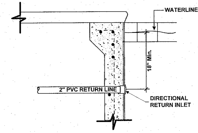
RETURN INLET DETAIL 3/4" = 1'-0"
