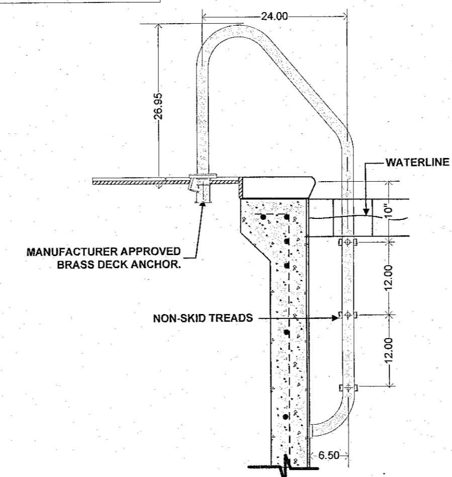
LADDER DETAIL 3/4" = 1'-0"
