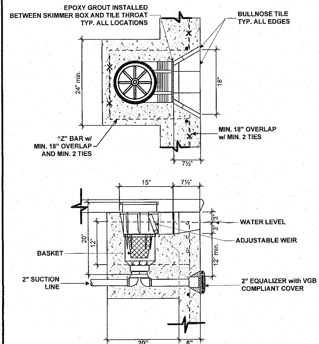
SURFACE SKIMMER DETAIL N.T.S.
