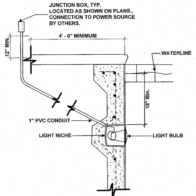
LIGHT DETAIL 3/4" = 1'-0"
