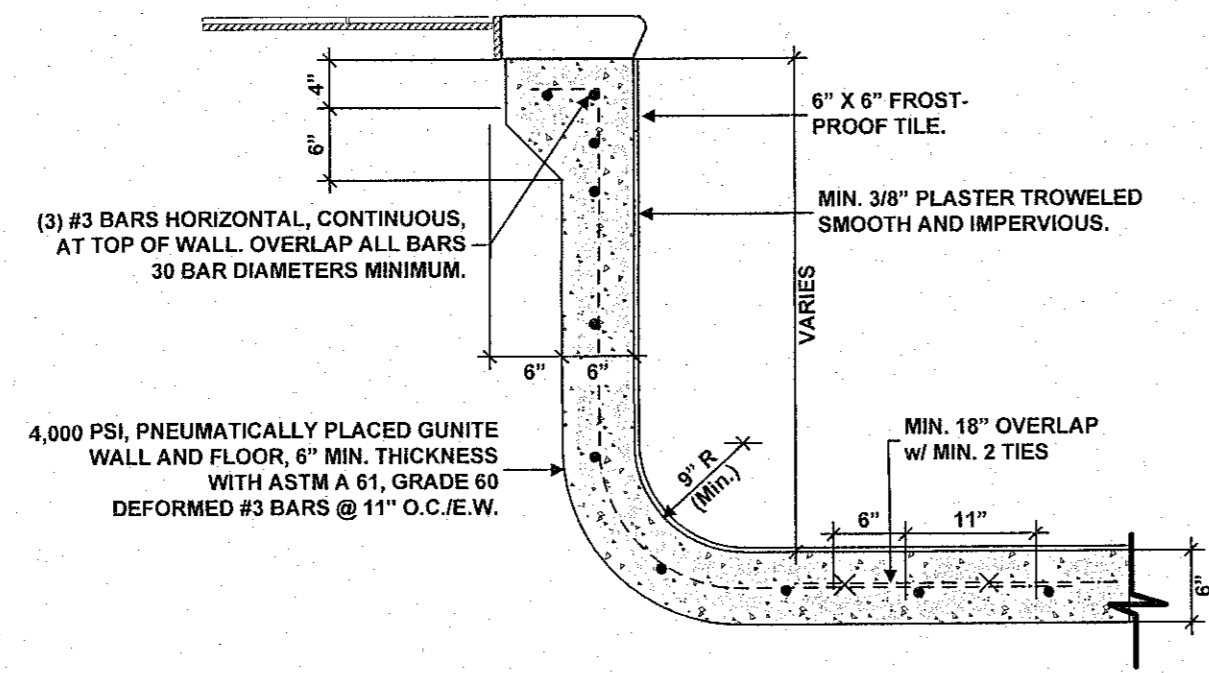
BOND BEAM DETAIL 3/4" = 1'-0"
